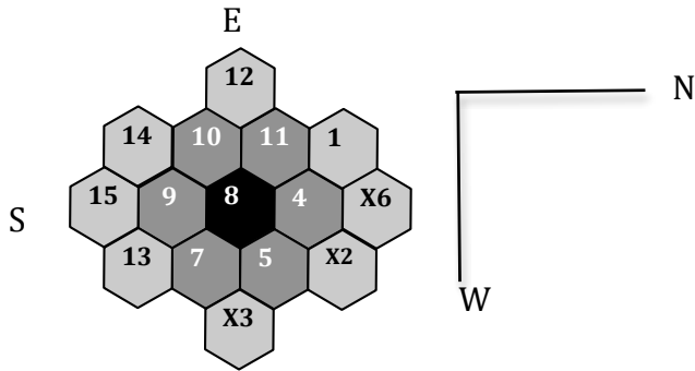
CYCLOPS Pseudo-slit Layout.
